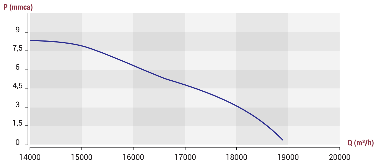
800 RPM
