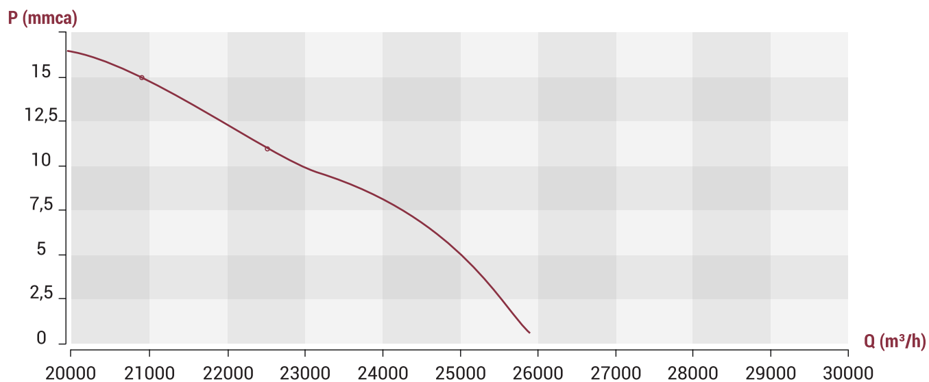
1100 RPM
